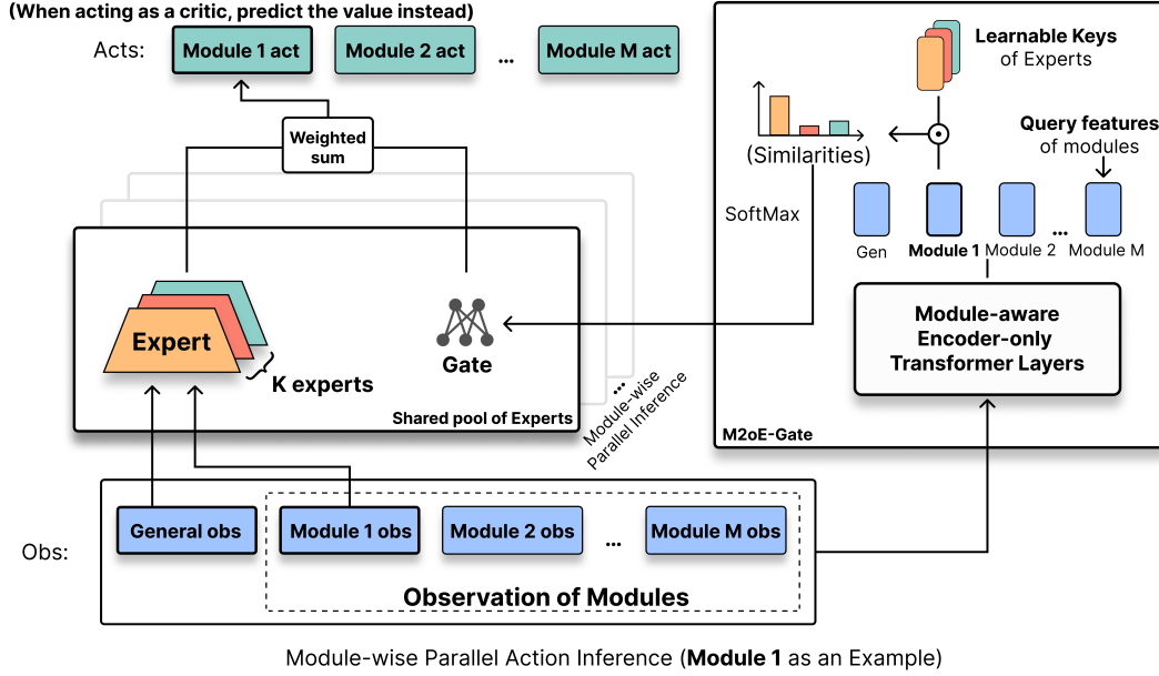
Fig. 3. Structure of Modular Mixture of Experts (M2oE). There are two main components: a module-wise shared pool of experts and an attention-based gating mechanism (M2oE-Gate) that extract inter-module correlations to select experts for each module. The design of M2oE enables module-wise parallelism and automatic adaptation to morphologies with different numbers of modules. This figure illustrates the action inference process for the first module in a robot with M modules.
