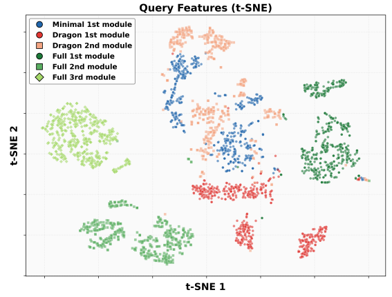
Fig. 7. t-SNE visualization of gating query features across morphologies. Each point represents a transformer output feature (query vector) produced by the gating network during forward locomotion at a fixed velocity command. Distinct clusters indicate that the gating network learns morphology- and module-specific representations in the shared embedding space, enabling expert selection across heterogeneous body structures.
